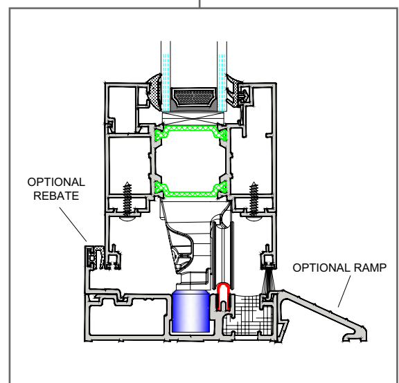
LOW THRESHOLD DETAIL
